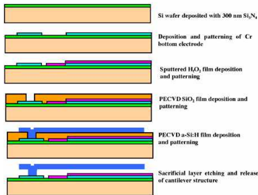
&lt;MEMS chip 제조공정&gt;
